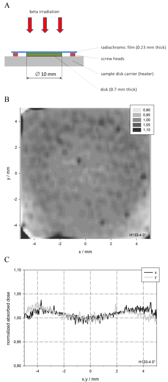
Figure 4: Experimental setup to mimic the irradiation of a sample on a flat disc in a lexsys reader. The geometry of the source mounting and film placement was identical to the actual situation in a reader by using e.g. an original heater plate on arm. (A) Geometry; (B) contour plot of normalised absorbed dose; (C) normalized absorbed doses for two profiles (for more details see Fig. 3 caption).
